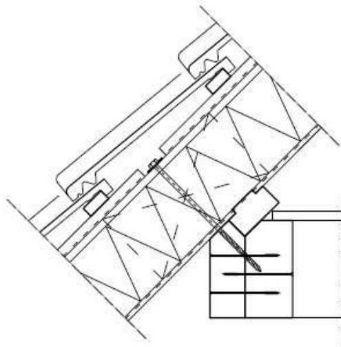
detail 11
