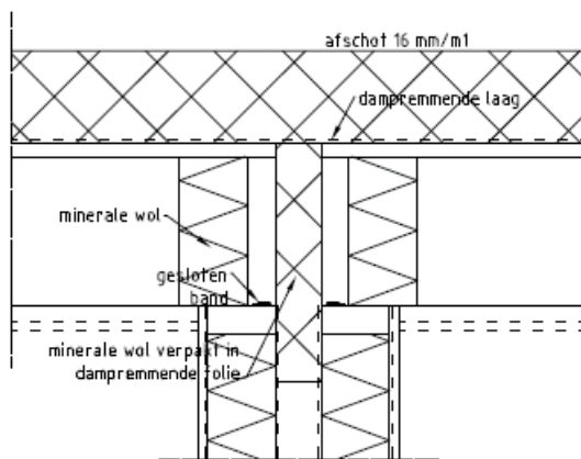
detail 8
