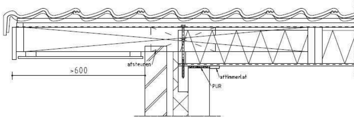
detail 12a
