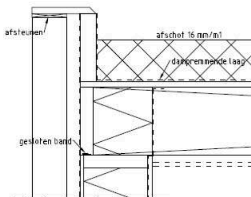
detail 7
