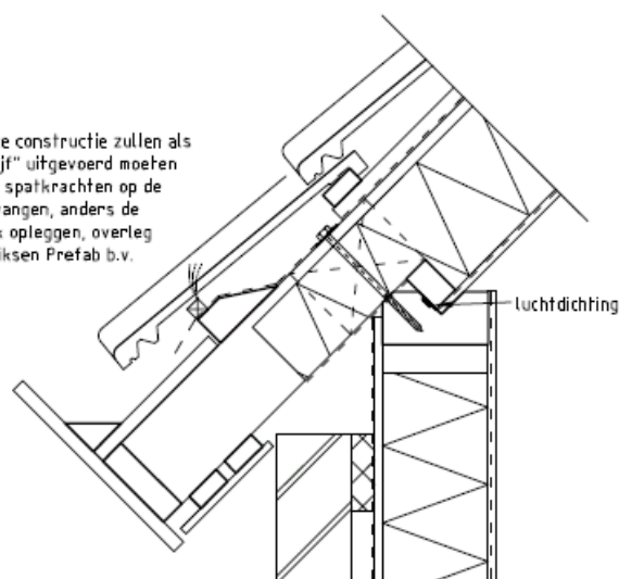
detail 10
