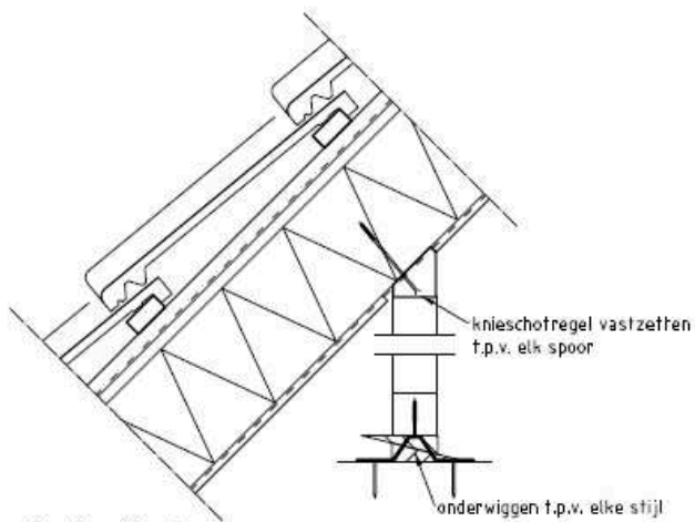
detail 6
