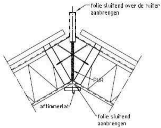
detail 19
