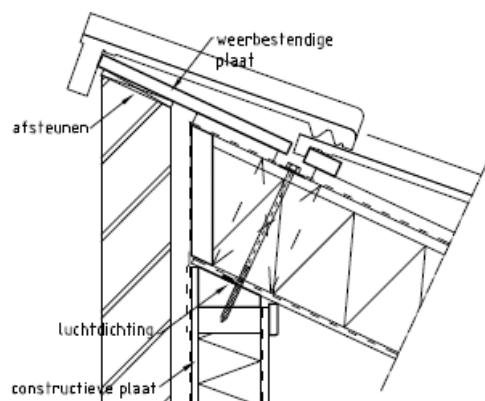
detail 9
