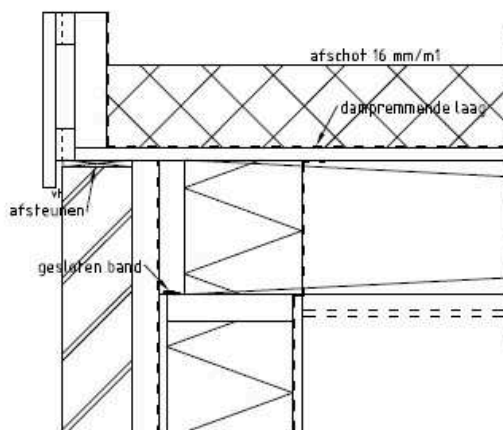
detail 7a
