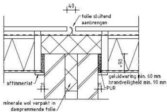
detail 3
