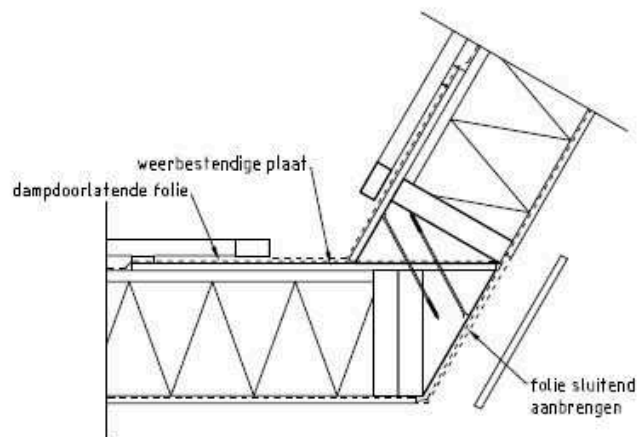
detail 20
