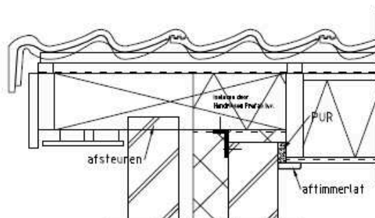
detail 12
